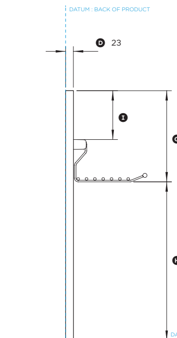
PROFILE VIEW
